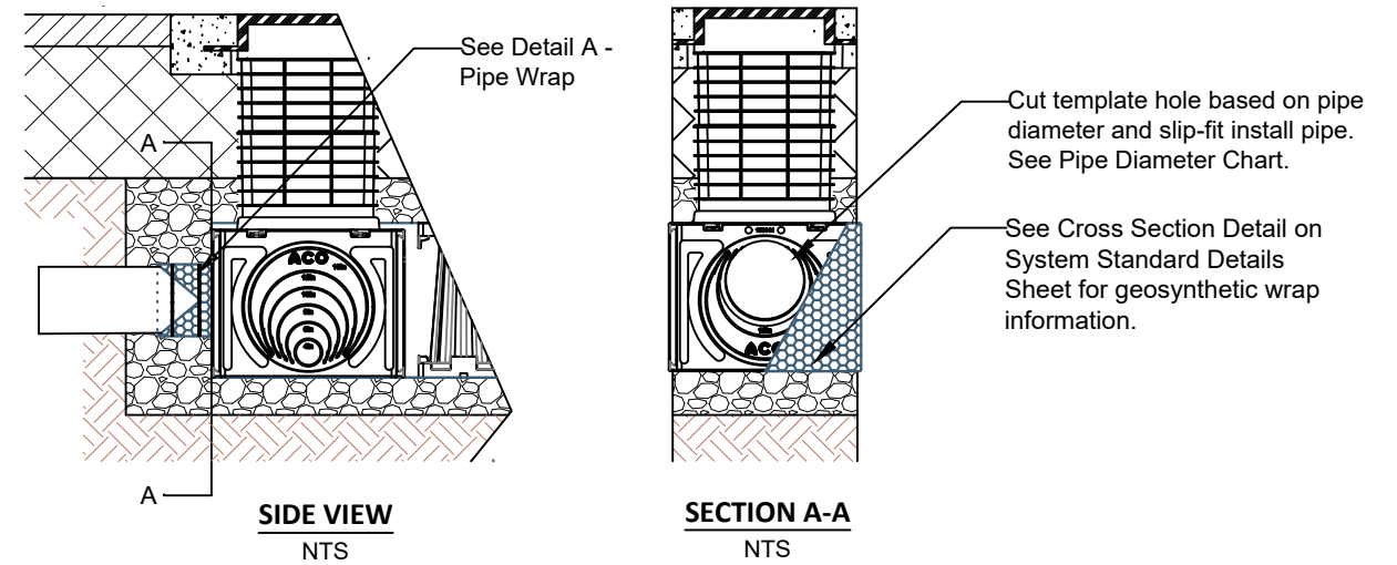
0.5 LAYER 900SD - REMOTE ACCESS UNIT PIPE INSTALLATION NTS
