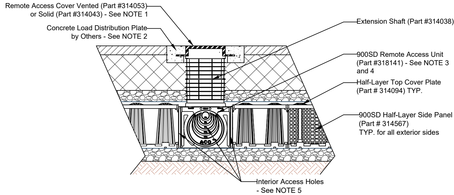
0.5 LAYER 900SD - REMOTE ACCESS UNIT ACCESS POINT CROSS SECTION NTS
